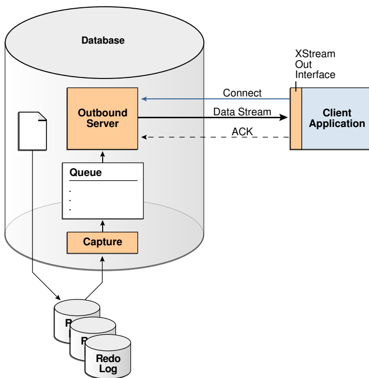
Figure 25-1 XStream Out
