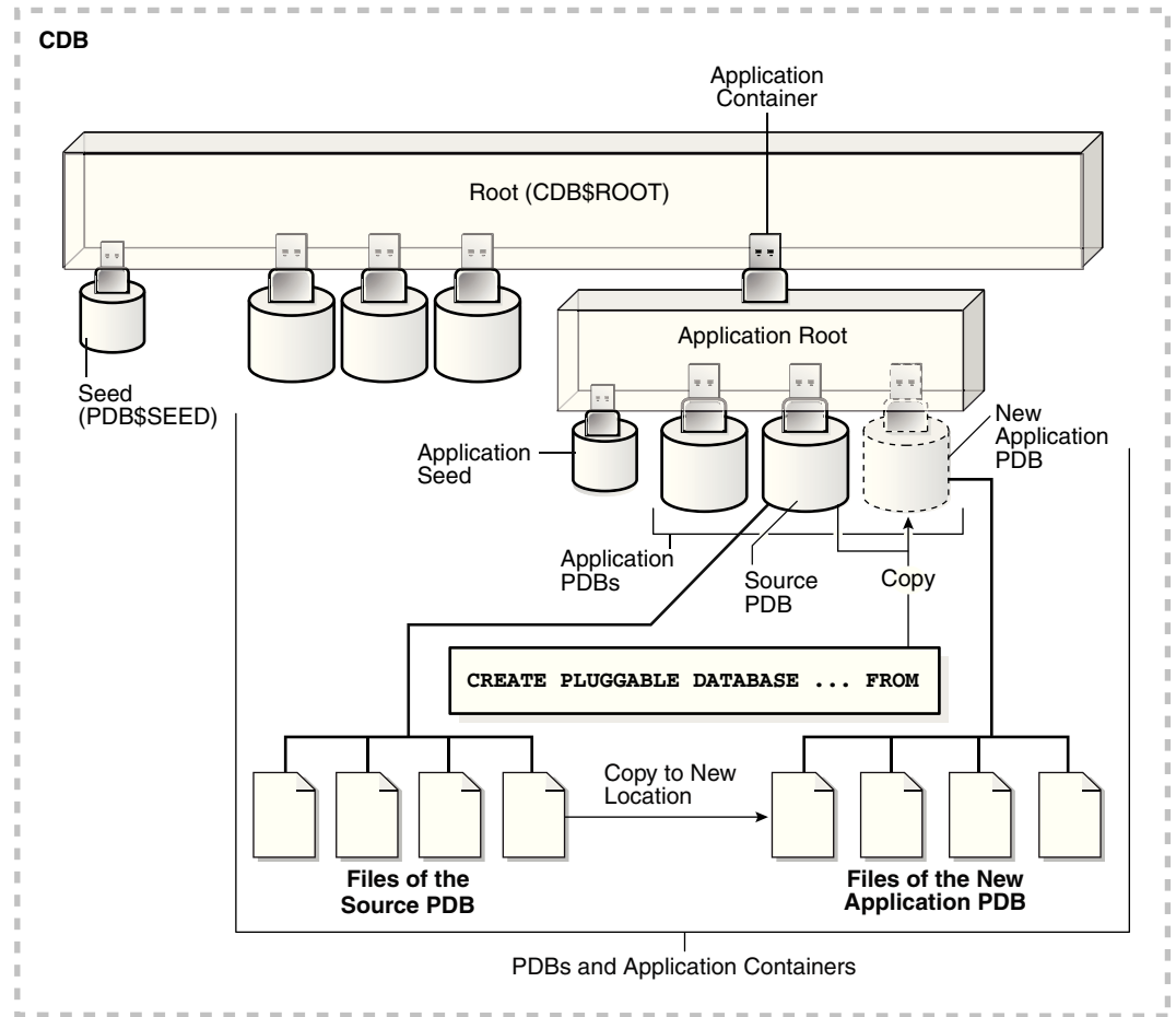
Figure 7-1 Clone a PDB in an Application Container
