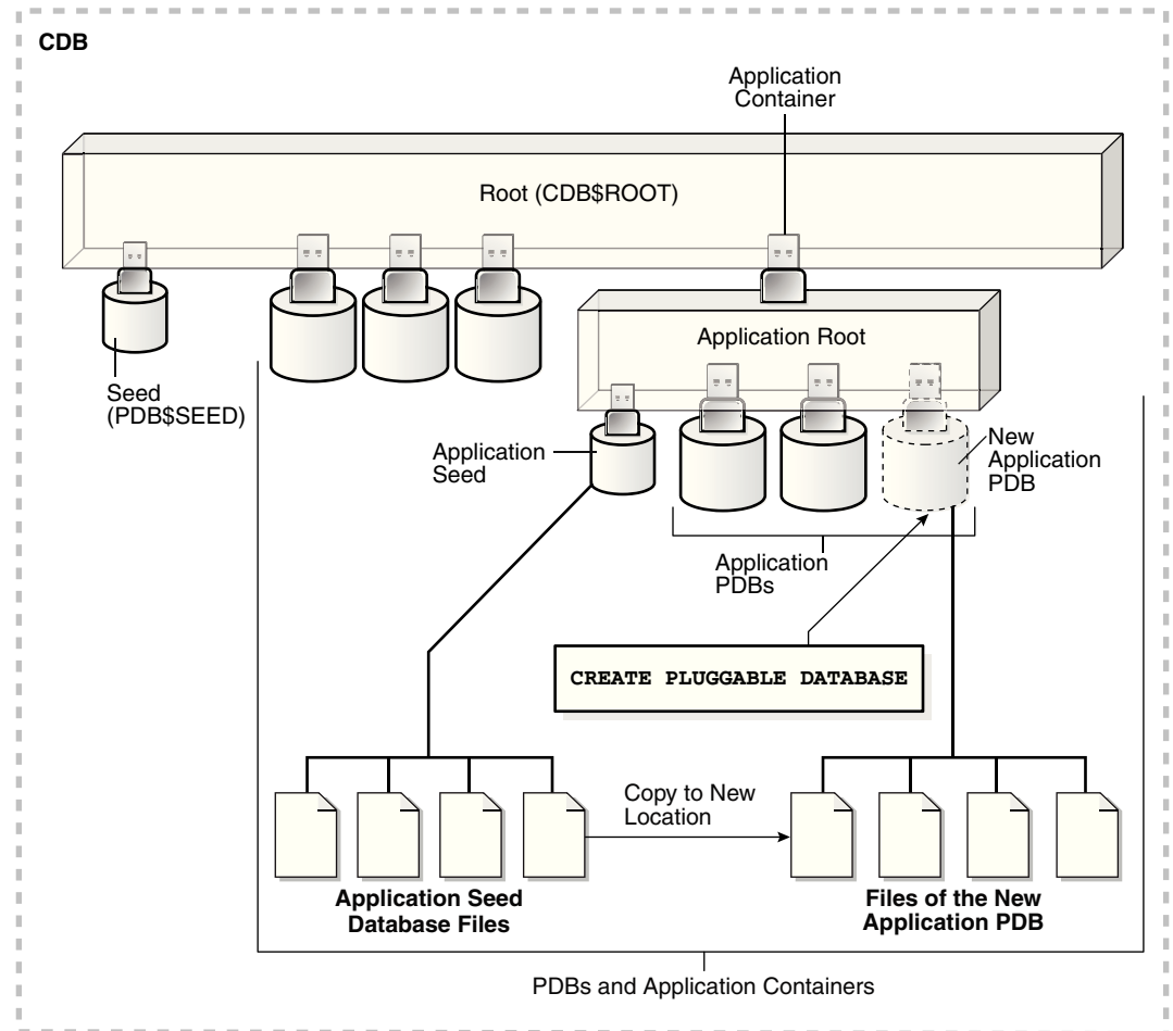
Figure 6-2 Create a PDB in an Application Root Using the Application Seed Files
